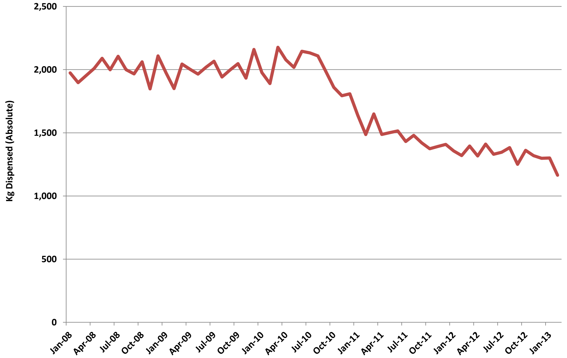
Monthly Kg Dispensed of Oxycodone ER January 2008 - February 2013
