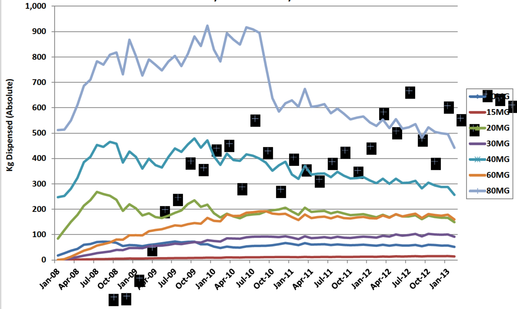
Monthly Kg Dispensed of OxyContin by Dosage Strength January 2008 - February 2013
